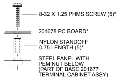
PCB MOUNTING DETAIL (*HARDWARE INCLUDED WITH 201678)
