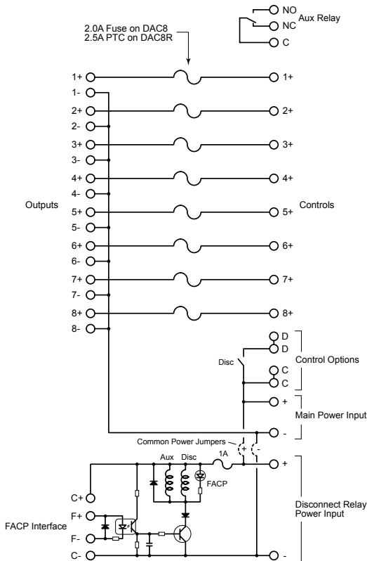
DAC8 / DAC8R Schematic Diagram
