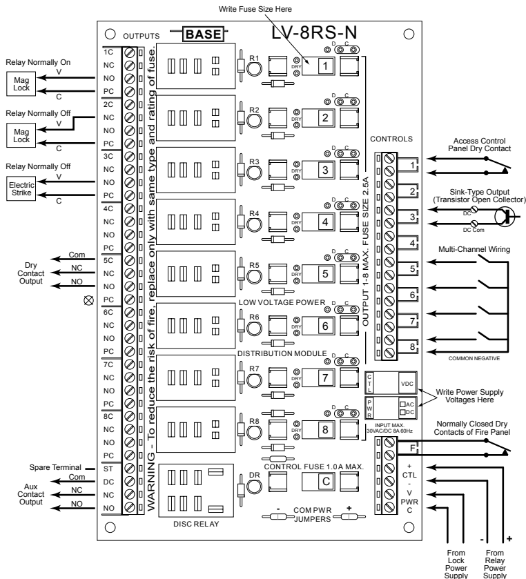
Figure 1 - LV-8RS-N Wiring Diagram
