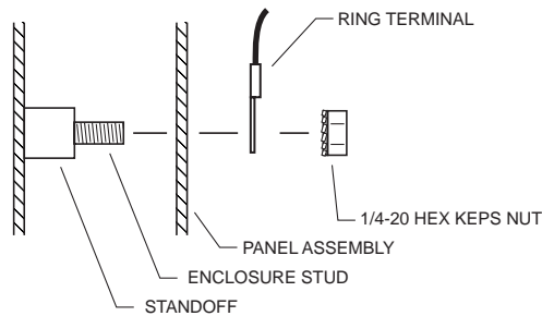
Figure 1. Panel and Ground Wire Installation
