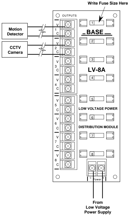
Figure 1 - LV-8A Wiring Diagram
