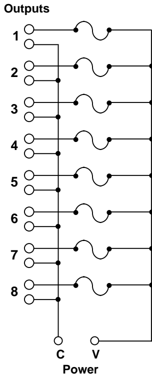
Figure 2 - LV-8A Schematic Diagram
