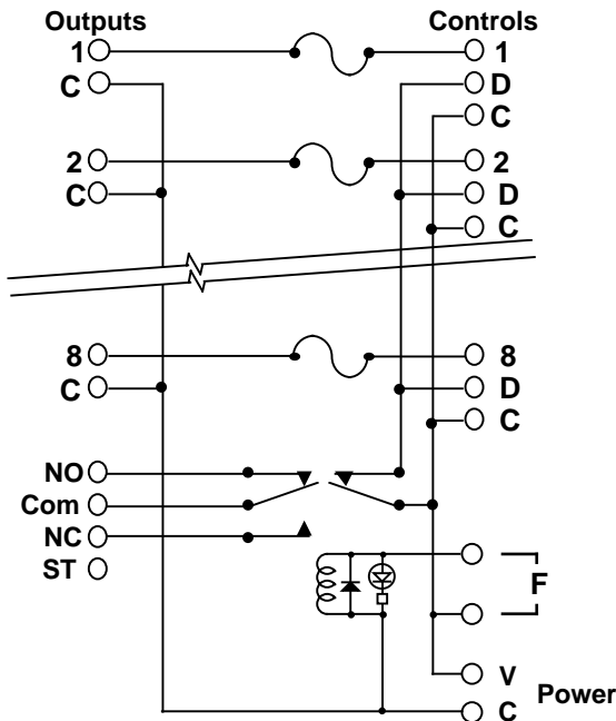
Figure 2 - LV-8S Schematic Diagram
